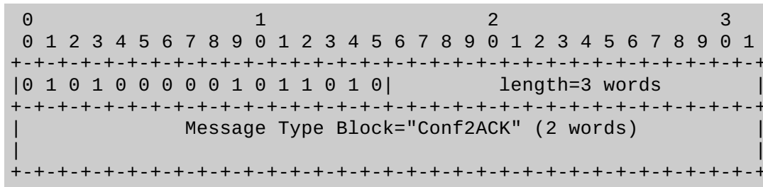
Figure 11: Conf2ACK Message Format
