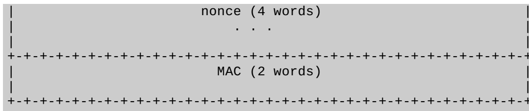
Figure 6: Multistream Commit Message Format
