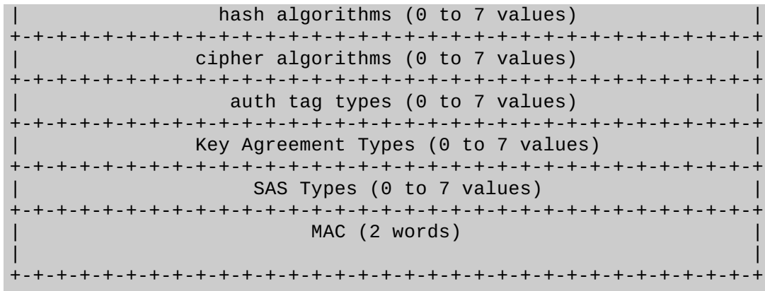
Figure 3: Hello Message Format
